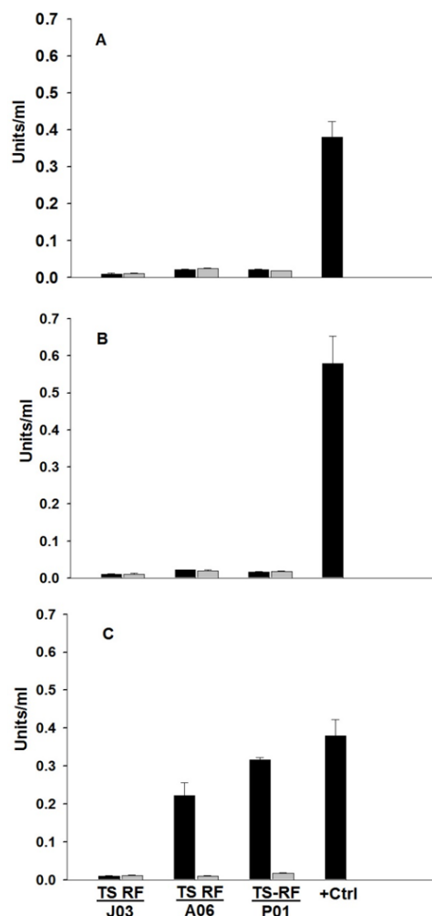
Figure 2: Calculated(A) chitobiosidase activity, (B) \beta -N-acetylglucosaminidase activity and(C) endochitinase activity of protein samples.
